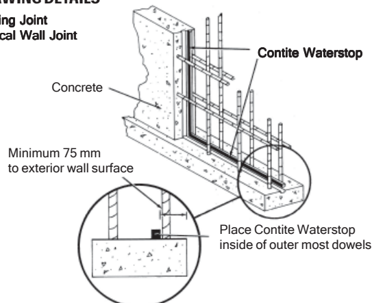
Typical placement of Contite Waterstop at concrete construction joints
