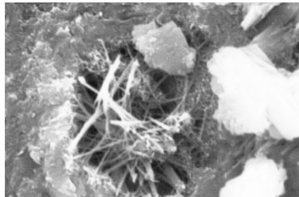
Crystals Forming Through A Void 350-400 μm in Width. Some damage is shown to the crystal through the coring process of the Sample. (Photograph has been taken 15 cm into the concrete)
