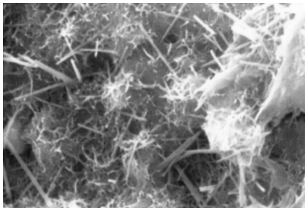
Fully developed crystal growth at 28 days within the capillary tracts of concrete blocking flow of water.
